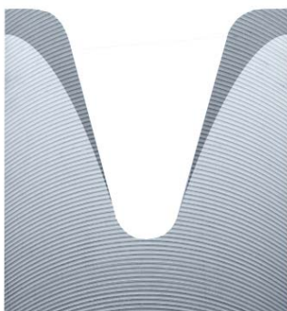
Bottom tool with WILA's proprietary CNC-Deephardenig® process applied.
