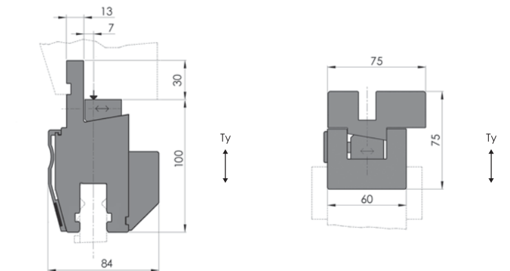
Example: Tool Holder with ES I adaption including Ty-alignment Example: Tool Holder with ES IV adaption including Ty-alignment
